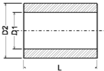
bushing without collar
