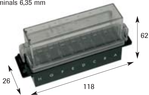
REF 123TA8392 For fuse: MED/RESET/FAST
