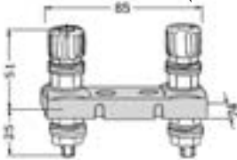
Fuse holder assy.: REF 106TA2693 For fuse: DIN 43560/43561
