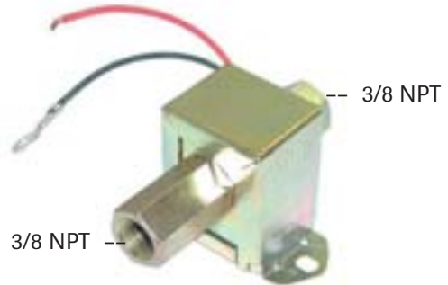
REF 115TA1806 12 V
