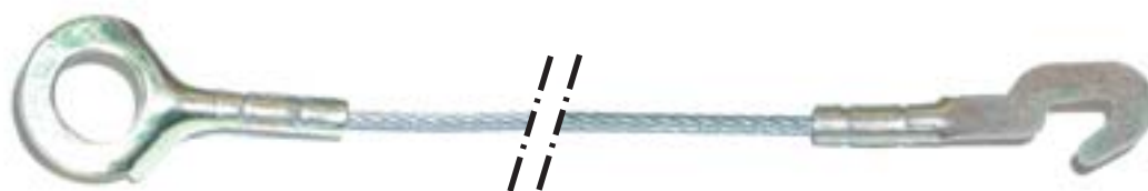
REF 106TA7012 cable length: 255 mm
