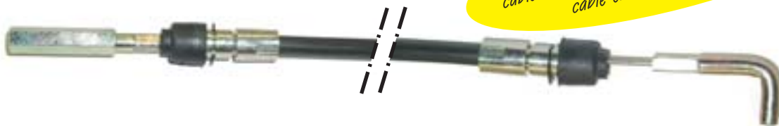
REF 106TA7020 cable length: 1570 mm
