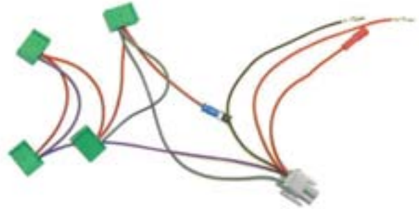
REF 118TA1831 Length: 365mm
